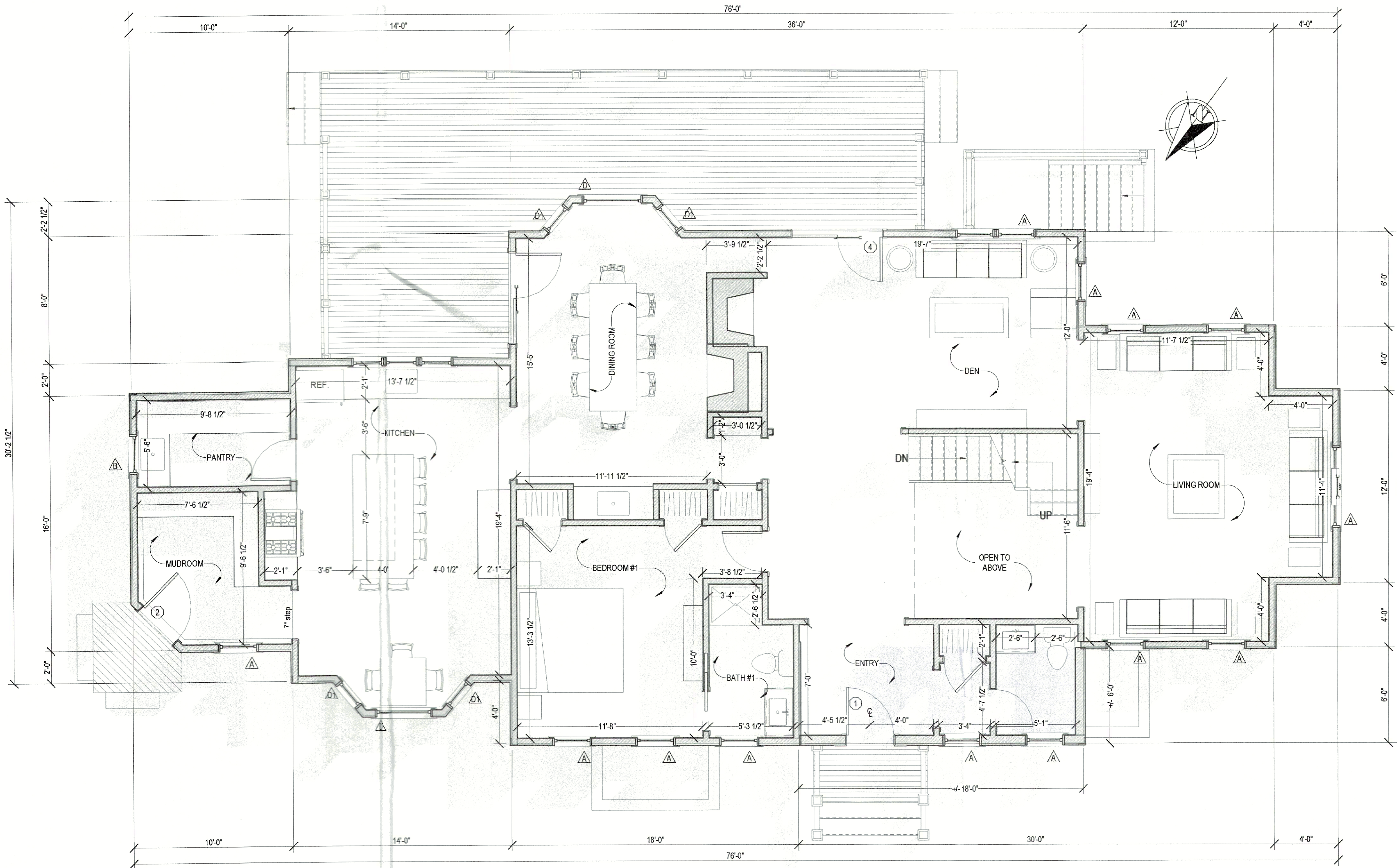
1 First Floor 1/4" = 1'-0"
