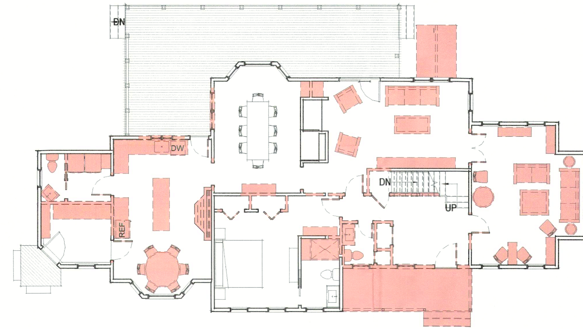
2 First Floor - Demo Plan 1/8" = 1'-0"
